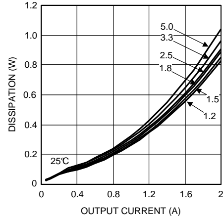
Figure 8. Dissipation 6-V Input at 25°C
