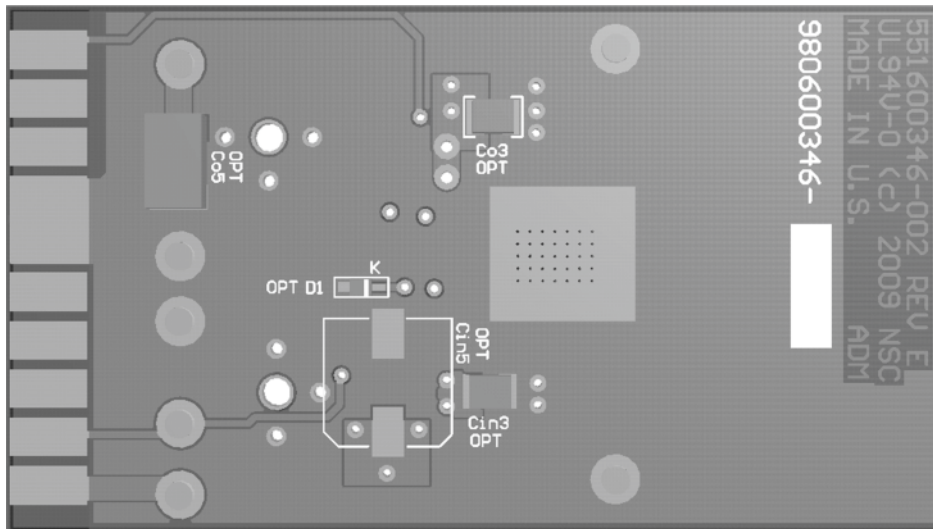
Figure 45. Bottom View of Evaluation PCB
