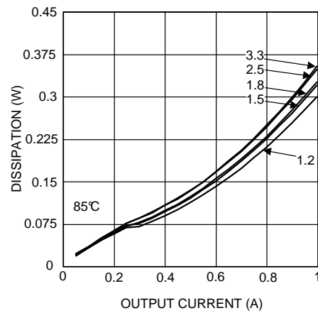
Figure 16. Dissipation 5-V Input at 85°C
