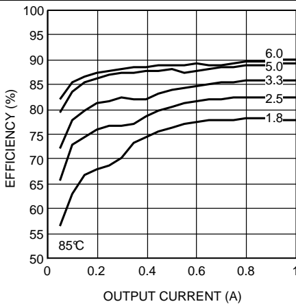
Figure 21. Efficiency 12-V Input at 85°C
