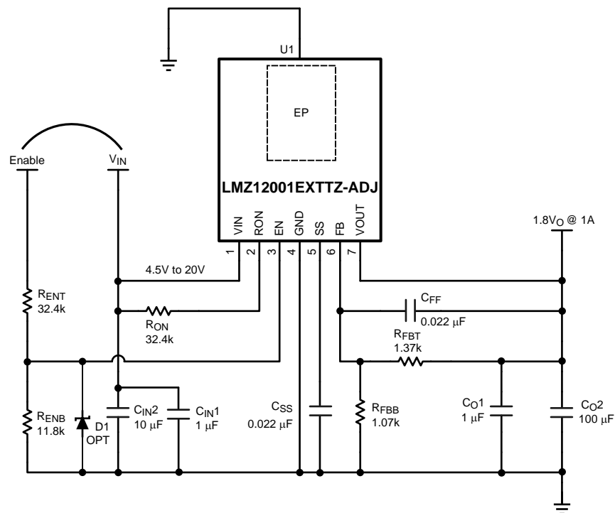
Figure 36. Evaluation Board Schematic Diagram
