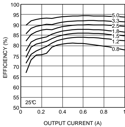
Figure 7. Efficiency 8-V Input at 25°C
