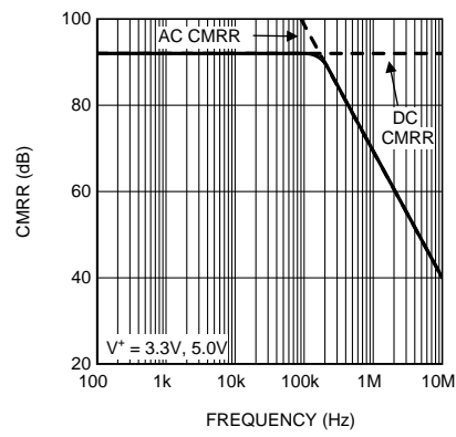
Figure 48. CMRR Curve
