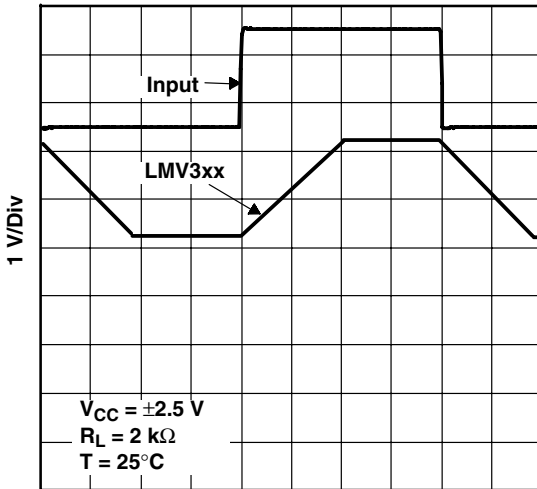
1 \mu\text{s}/\text{Div} Figure 27
