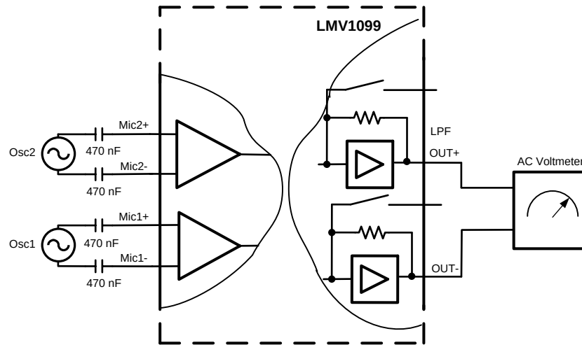
Figure 4. FFNS E , NFSL E , SNRI E Test Circuit
