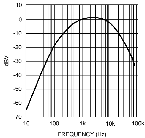
Figure 35. A-Weighted Filter
