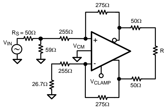
Figure 57. Single Ended Input S-Parameter Test Circuit (50Ω System)
