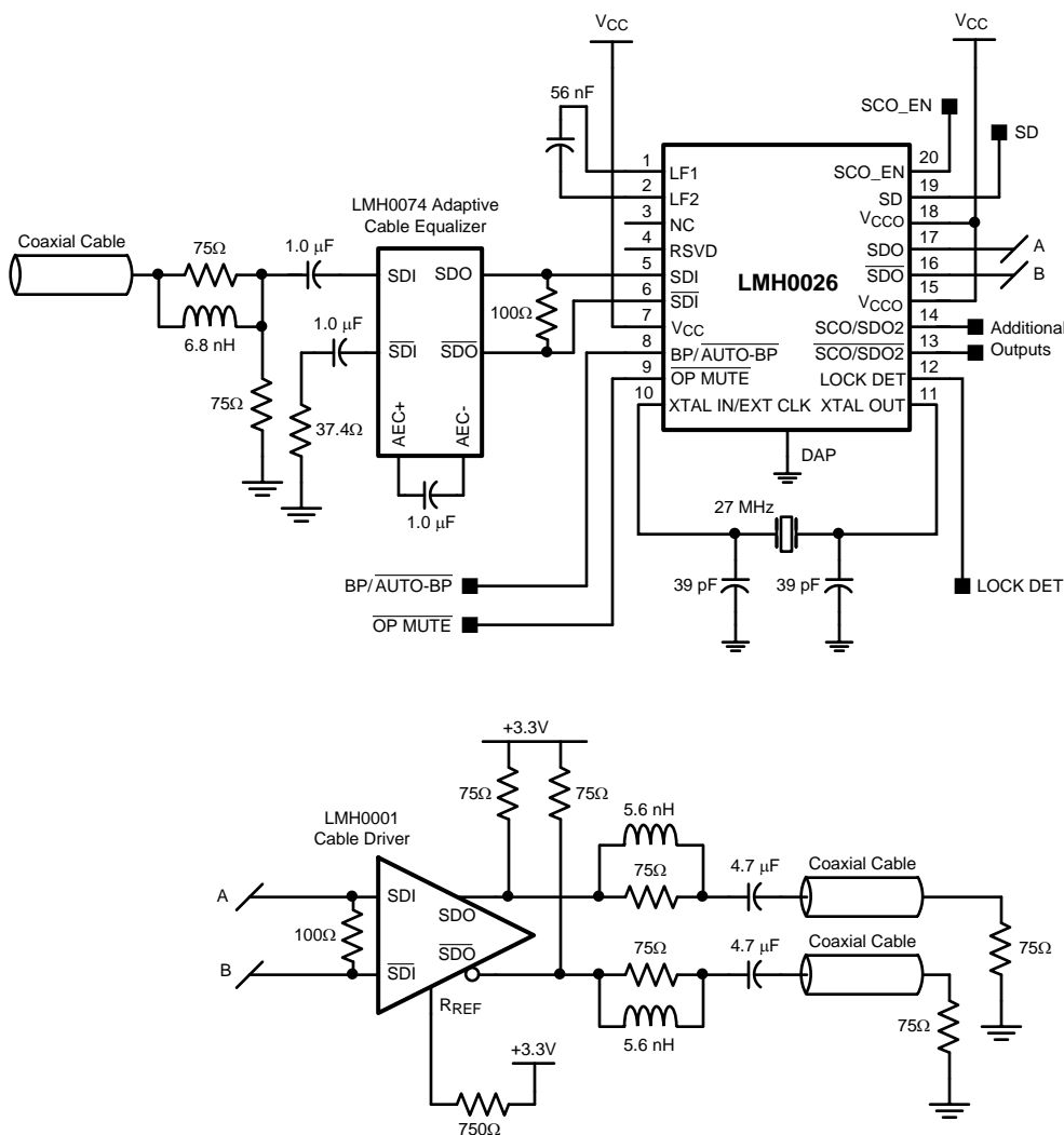
Figure 5. Application Circuit
