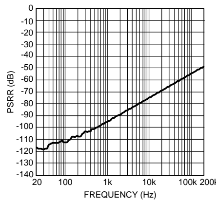
Figure 62. PSRR- vs Frequency V_{CC} = 15V , V_{EE} = -15V R_L = 600\Omega , F = 200kHz , V_{RIPPLE} = 200mvpp
