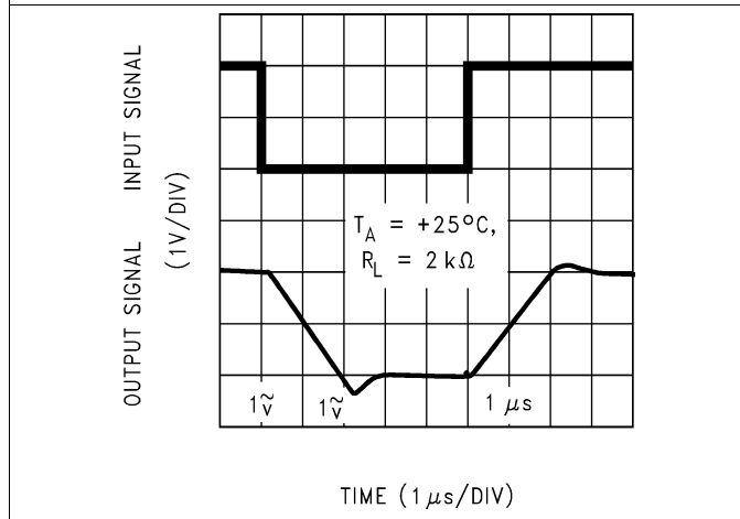
Figure 53. Noninverting Large Signal Pulse Response
