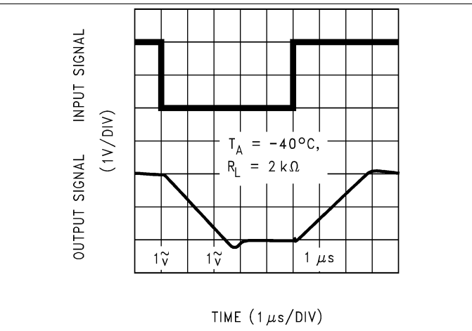
Figure 52. Noninverting Large Signal Pulse Response
