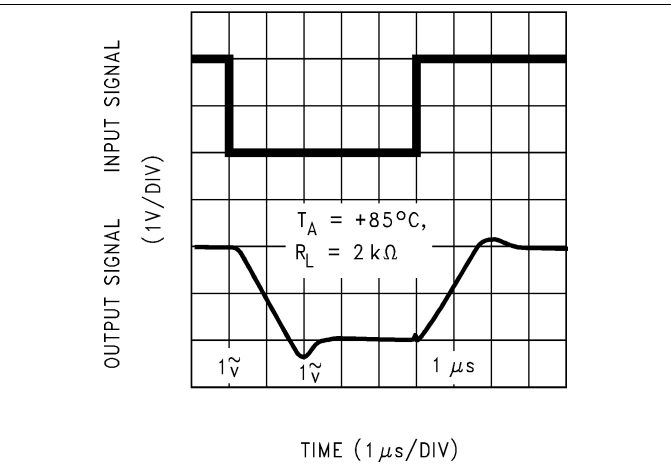
Figure 54. Noninverting Large Signal Pulse Response
