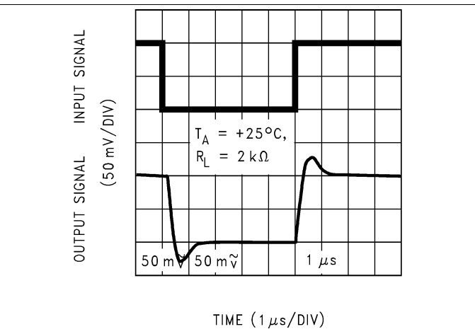
Figure 50. Noninverting Small Signal Pulse Response
