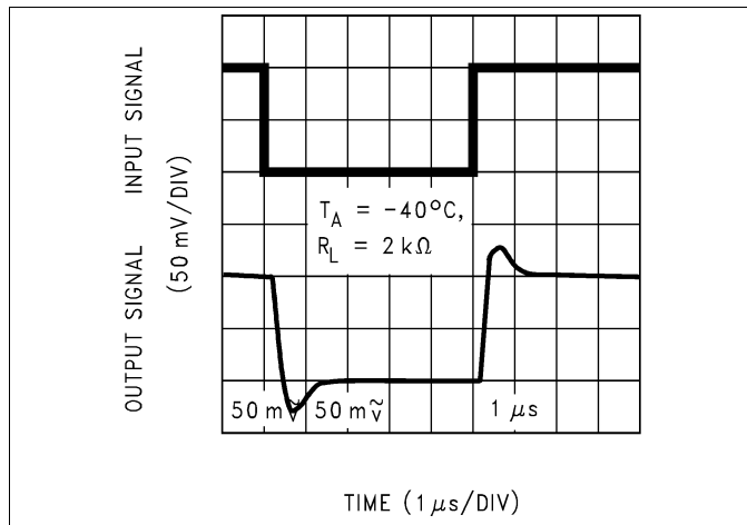
Figure 49. Noninverting Small Signal Pulse Response
