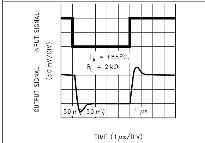
Figure 51. Noninverting Small Signal Pulse Response
