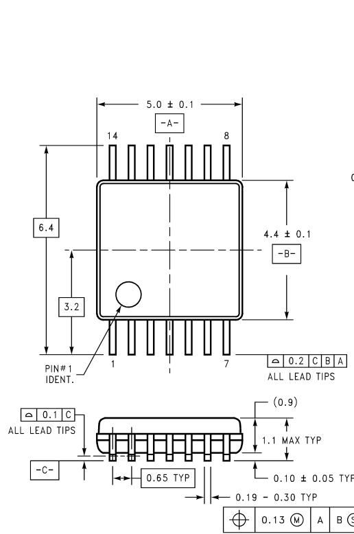
14-Pin TSSOP NS Package Number MTC14
