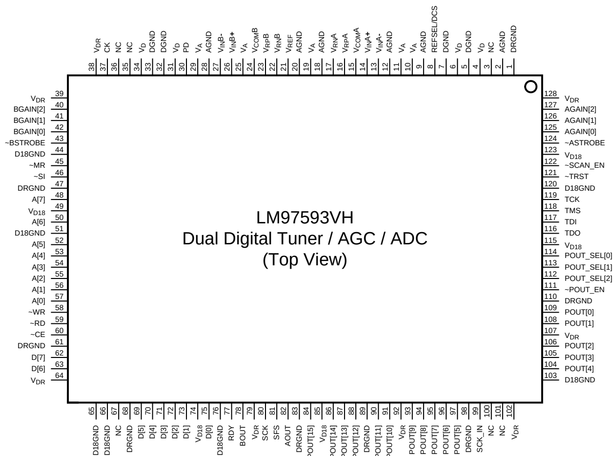
Figure 2. LM97593VH PQFP Pinout
