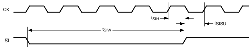
Figure 5. LM97593 Synchronization Input (SI) Timing
