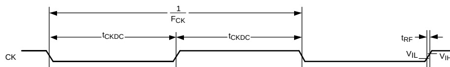
Figure 6. LM97593 Clock Timing
