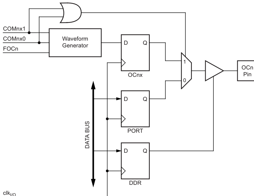
Figure 11-4. Compare Match Output Unit, Schematic
