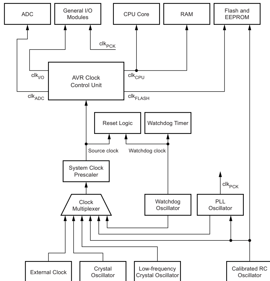
Figure 5-1. Clock Distribution
