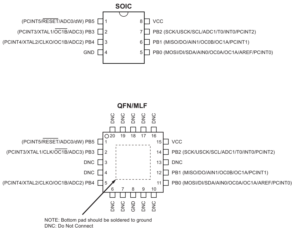
Figure 1. Pinout ATtiny25/45/85
