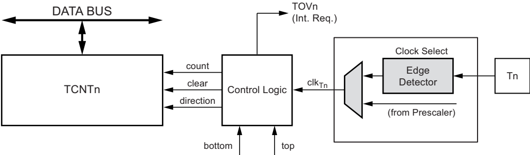
Figure 11-2. Counter Unit Block Diagram
