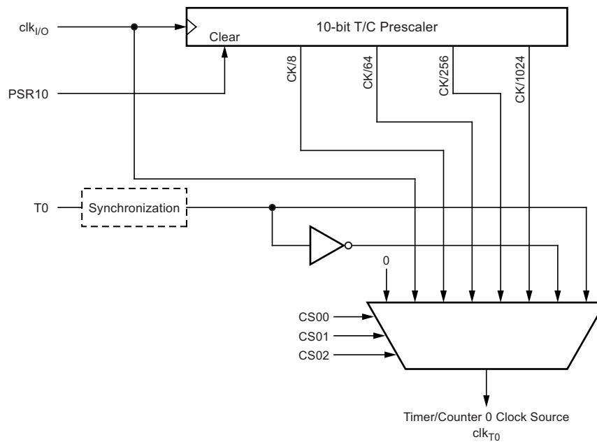
Figure 12-2. Prescaler for Timer/Counter0
