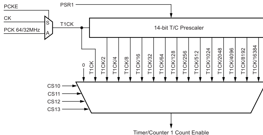
Figure 13-1. Timer/Counter1 Prescaler
