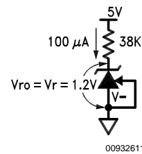
FIGURE 3. 1.2V Reference
