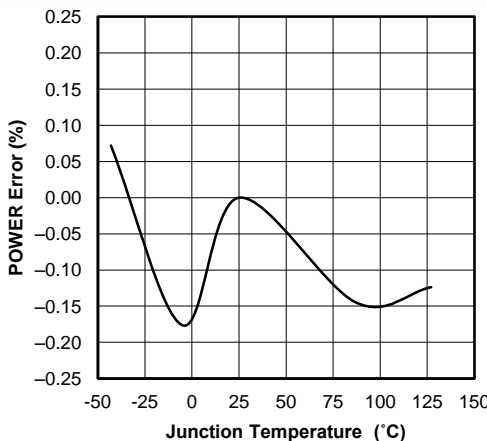
Figure 10. PIN Measurement Error ( V_{IN\_K} - SENSE = 22\text{ mV} )
