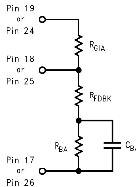
Figure 54. Low Frequency Enhancement ( MT/MH PINOUT )
