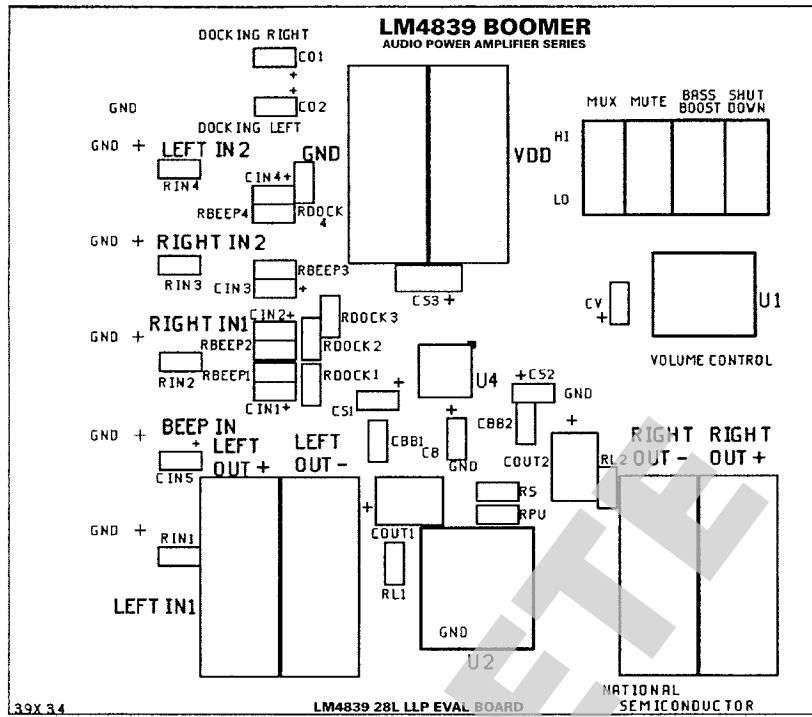
FIGURE 3. Recommended LQ PC Board Layout:Component-Side Silkscreen
