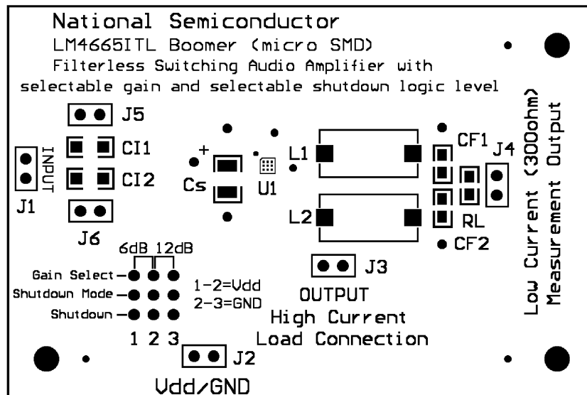
Figure 45. Silk Screen
