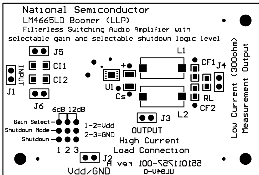
Figure 41. Silk Screen
