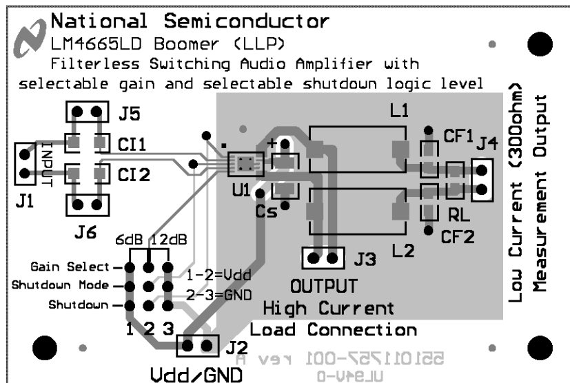
Figure 41. Silk Screen
