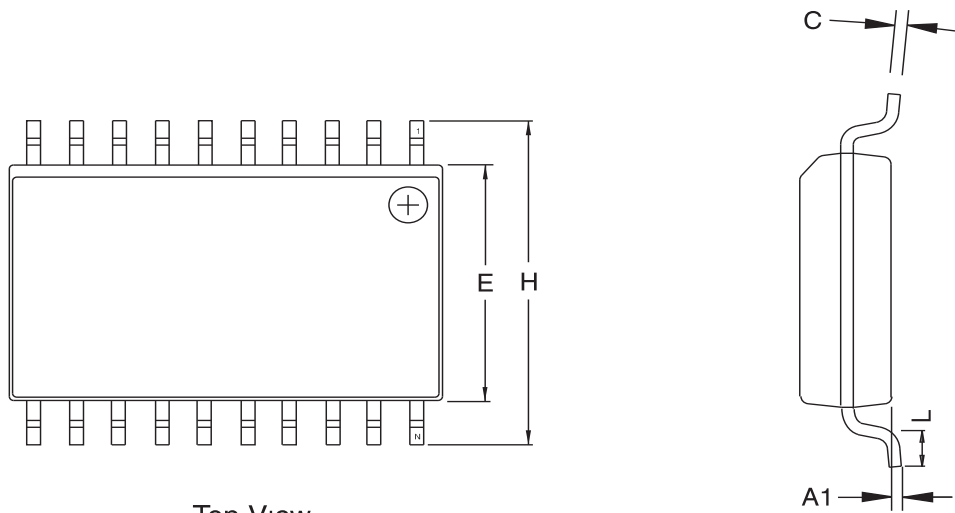
End View
