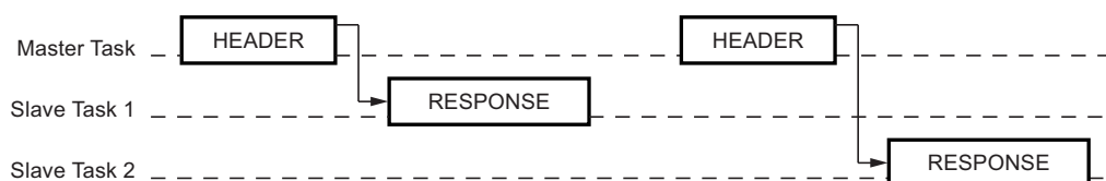
Figure 15-2. Master and Slave Tasks Behavior in LIN Frame
