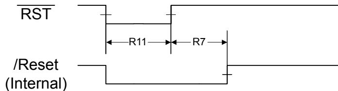
Figure 21-5. External Reset Timing ( \overline{RST} )
