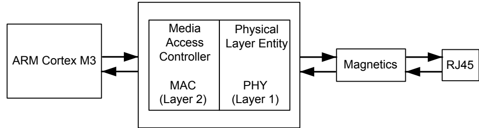
Figure 15-1. Ethernet Controller
