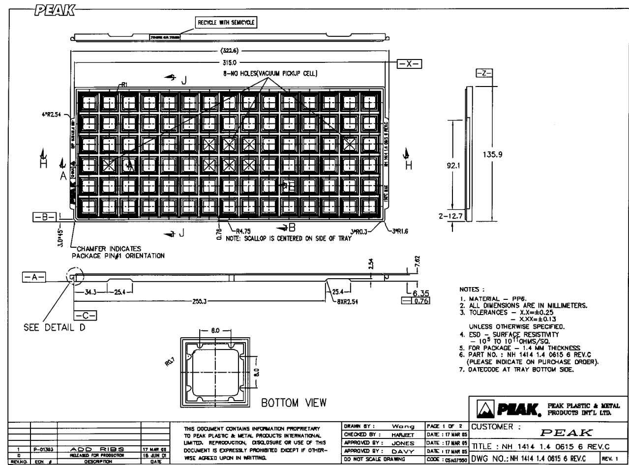
Figure E-2. 100-Pin LQFP Tray Dimensions
