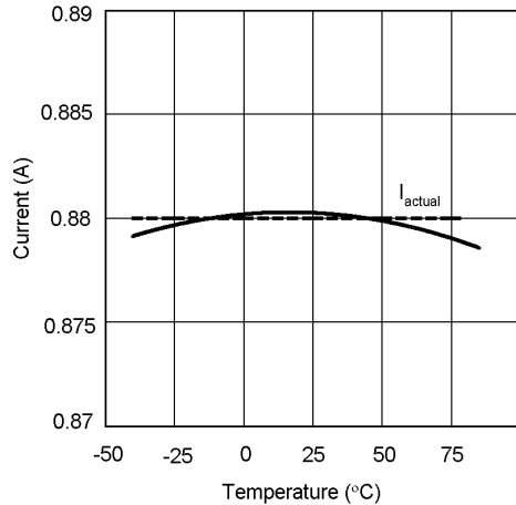
Accuracy vs Temperature (LM3822-1.0)
