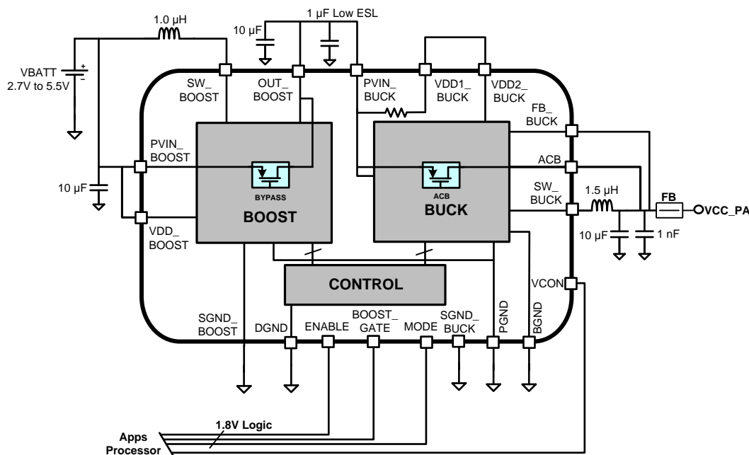
Figure 27. Typical Application: Boost-Buck
