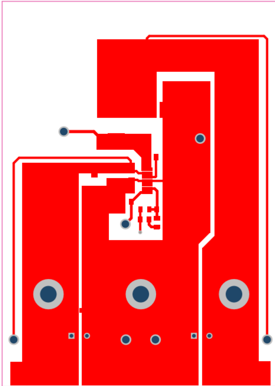
Figure 4. Top Layer Routing
