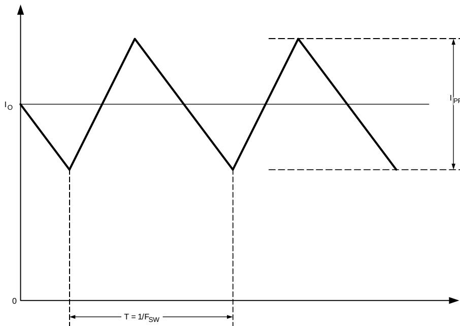
Figure 22. Inductor Current
