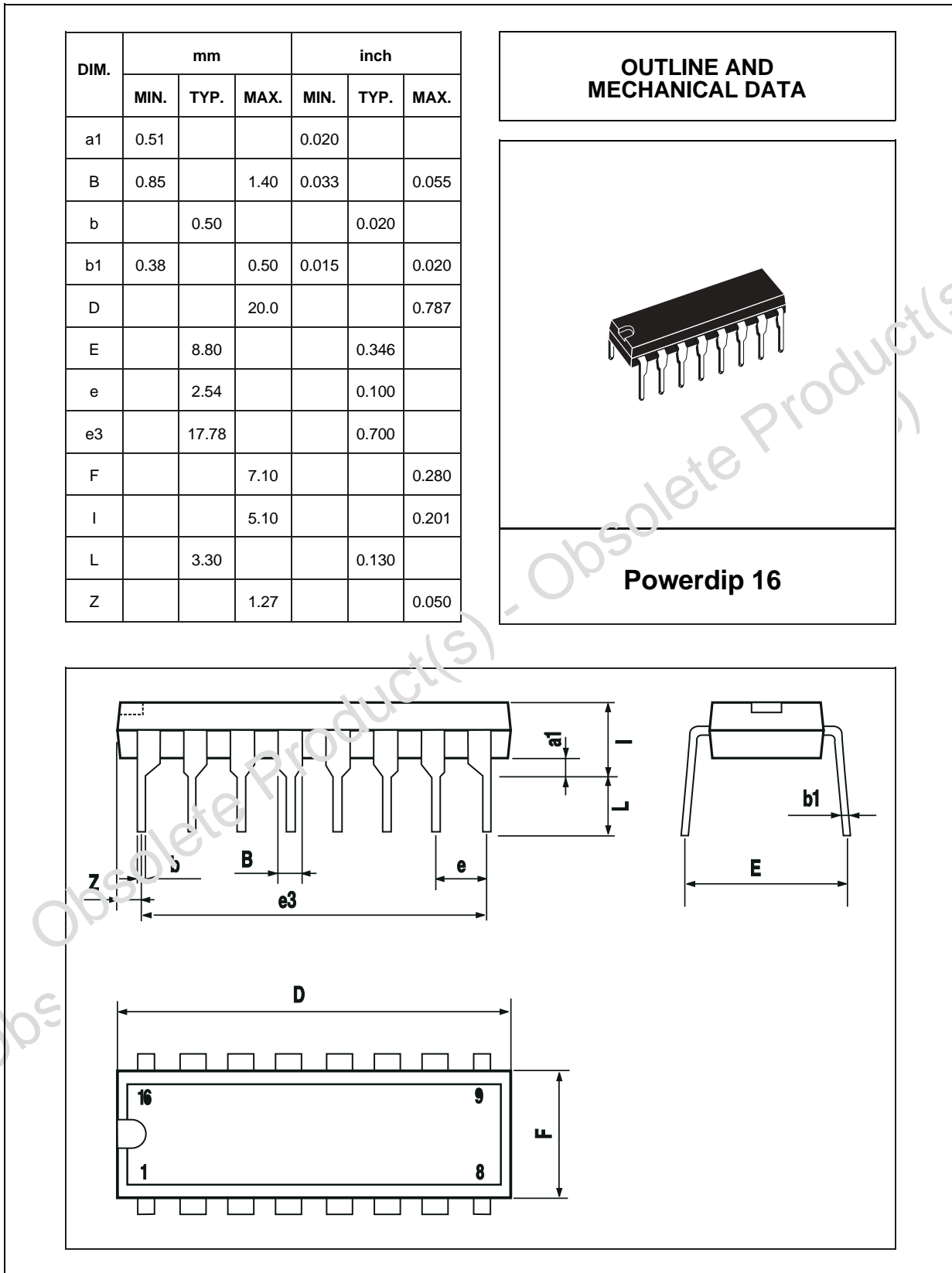
Figure 4. Powerdip (12+2+2) Mechanical Data & Package Dimensions
