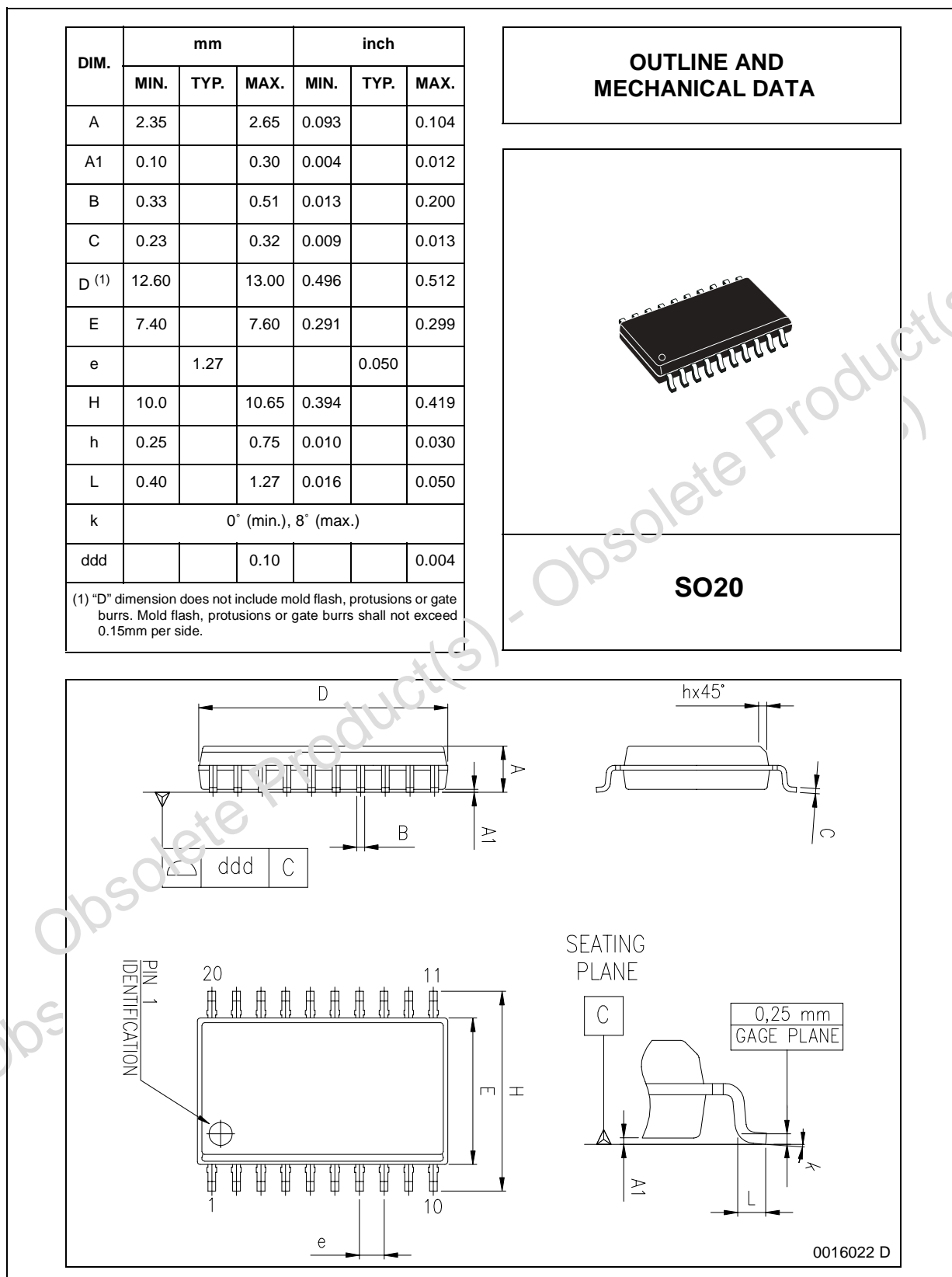
Figure 5. SO20L Mechanical Data & Package Dimensions
