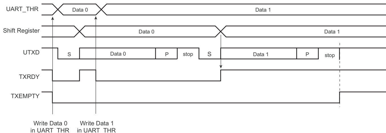
Figure 43-10. Transmitter Control
