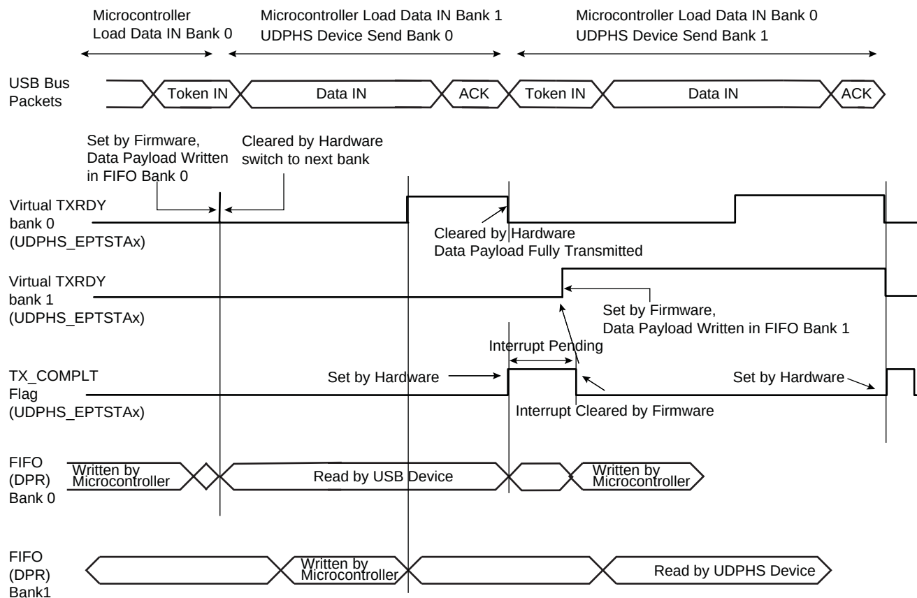
Figure 34-10.Data IN Transfer for Endpoint with Two Banks
