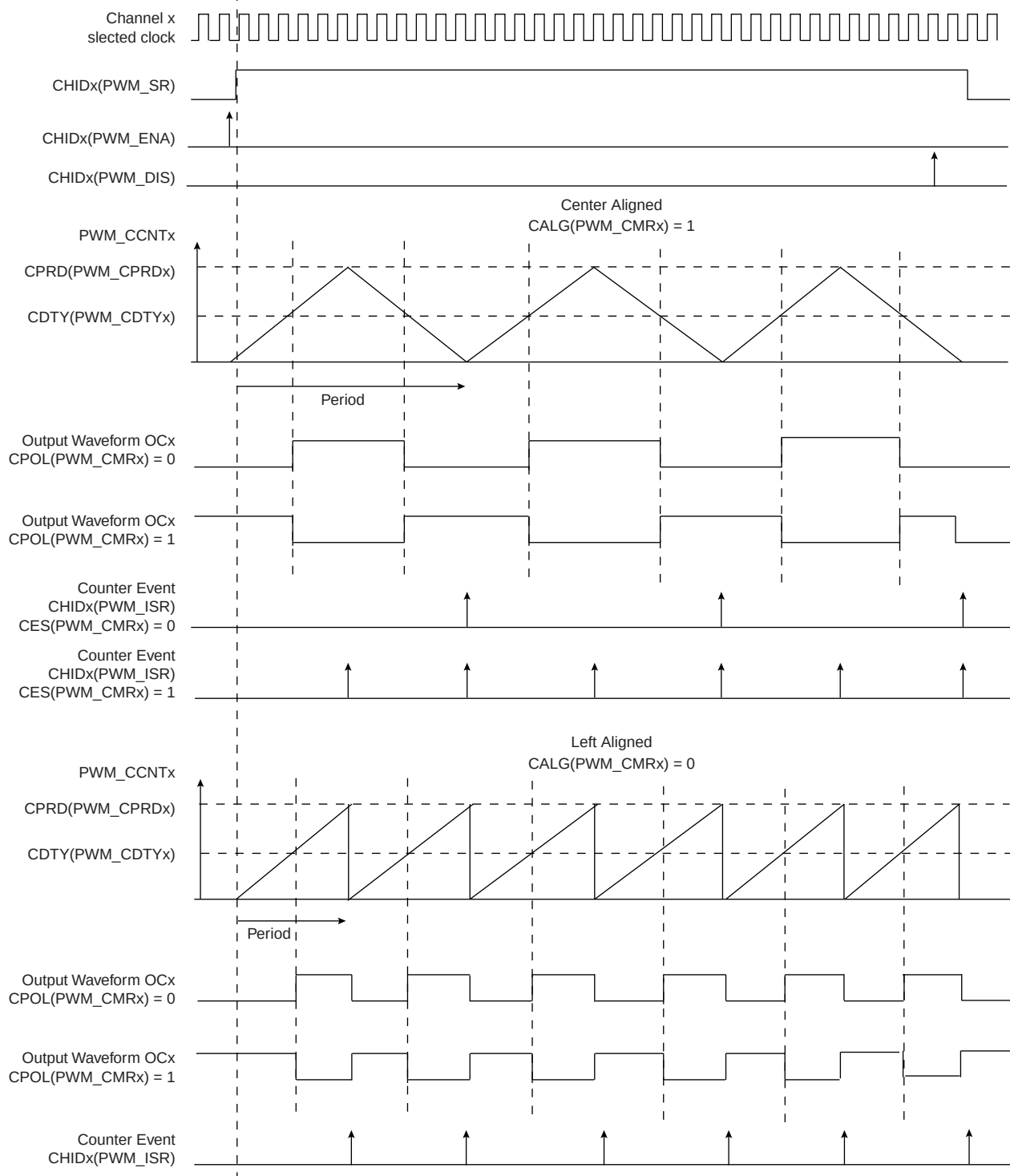
Figure 48-5. Waveform Properties
