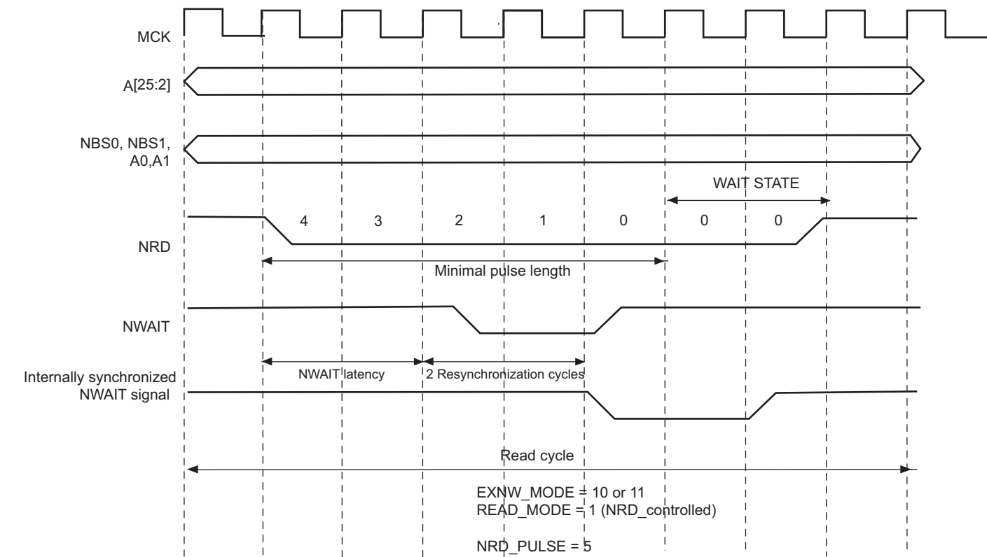
Figure 30-27.NWAIT Latency
