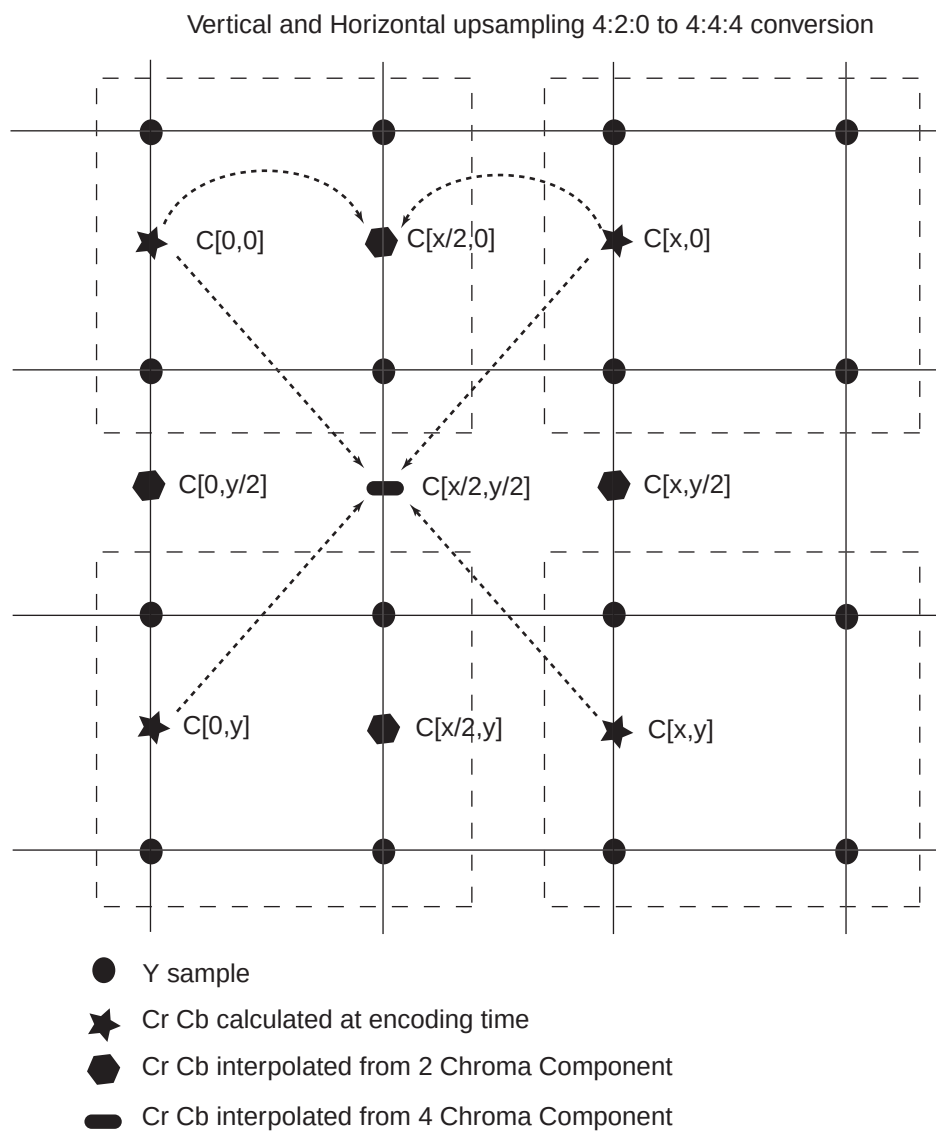
Figure 32-5. 4:2:0 Upsampling Algorithm
