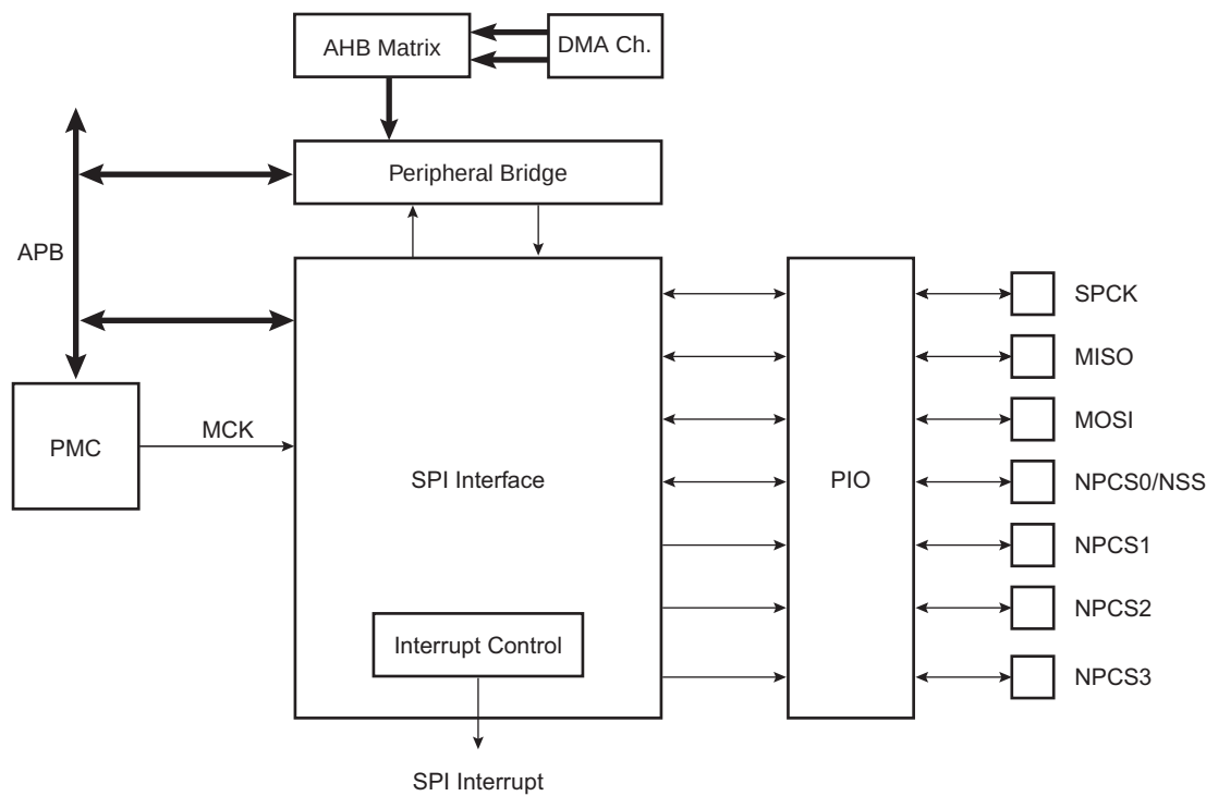
Figure 39-1. Block Diagram
