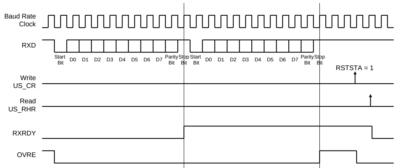
Figure 34-21. Receiver Status
