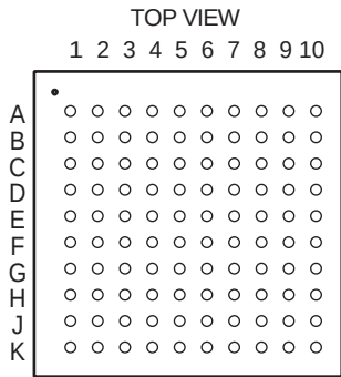
Figure 4-4. Orientation of the 100-ball TFBGA Package
