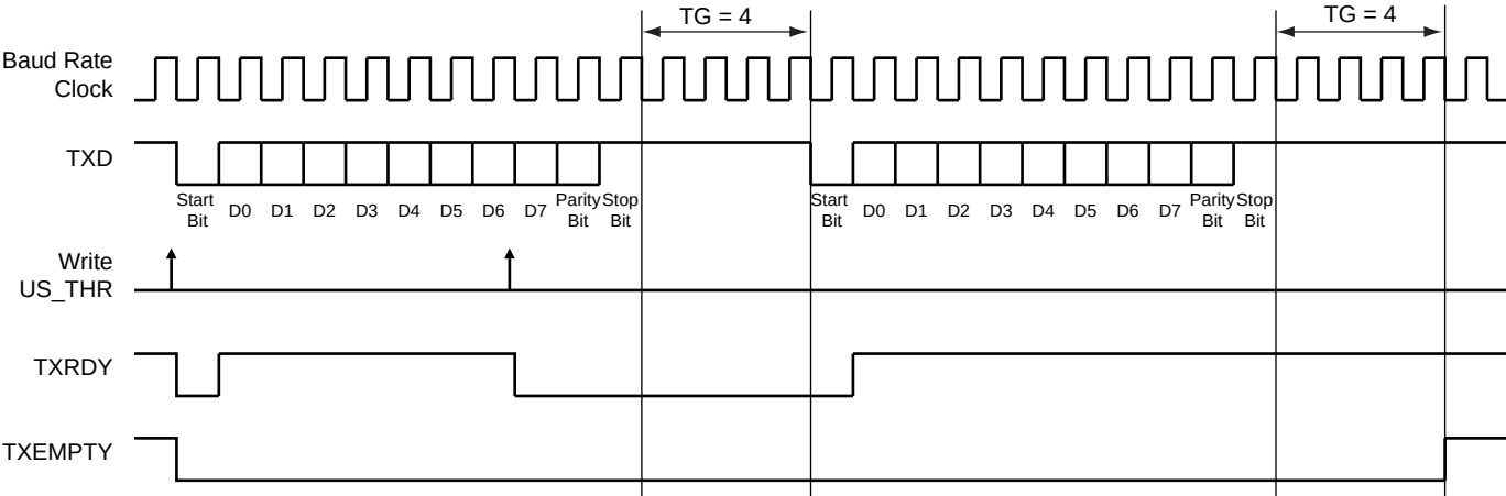
Figure 34-23. Timeguard Operations
