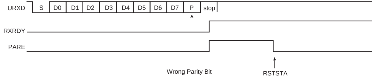
Figure 33-7. Parity Error
