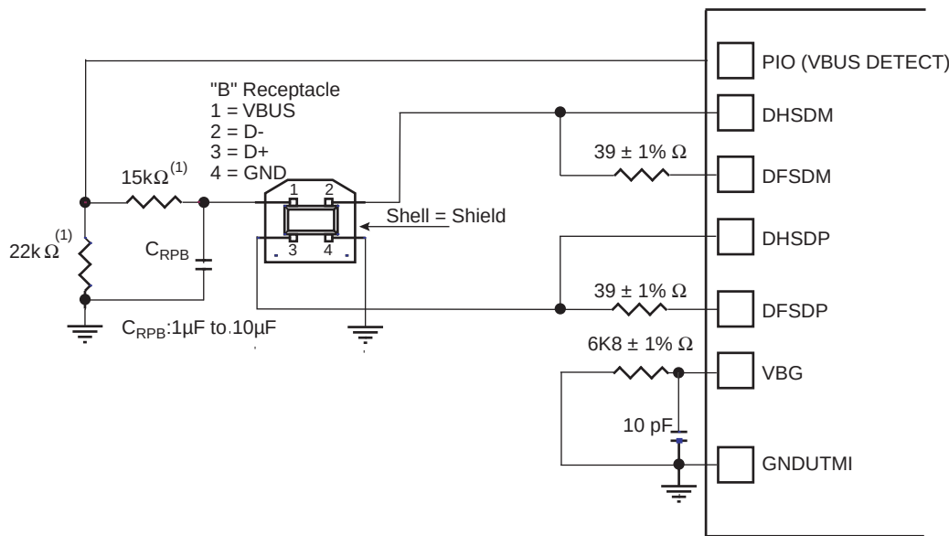
Figure 38-2. Board Schematic
