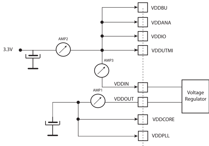
Figure 42-8. Measurement Setup for Wait Mode
