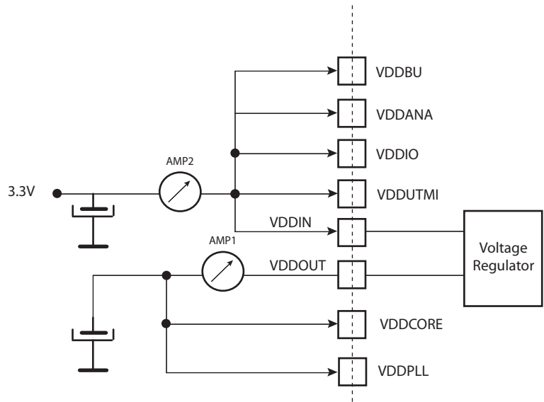
Figure 42-6. Measurement Setup for Sleep Mode
