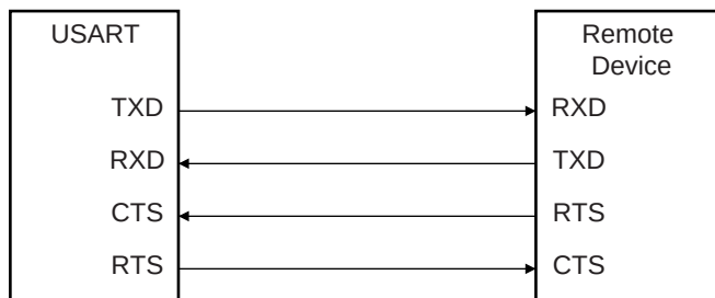
Figure 34-27. Connection with a Remote Device for Hardware Handshaking
