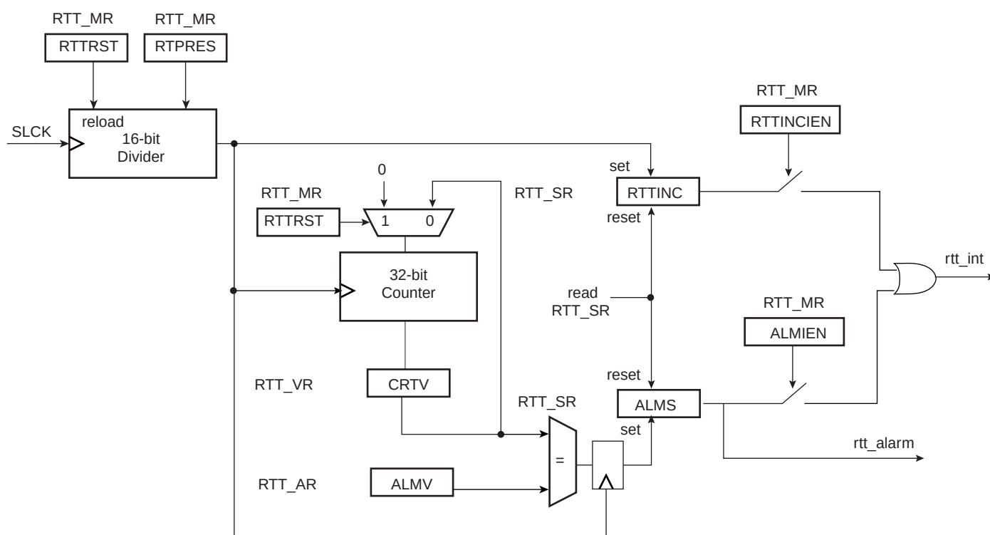
Figure 16-1. Real-time Timer
