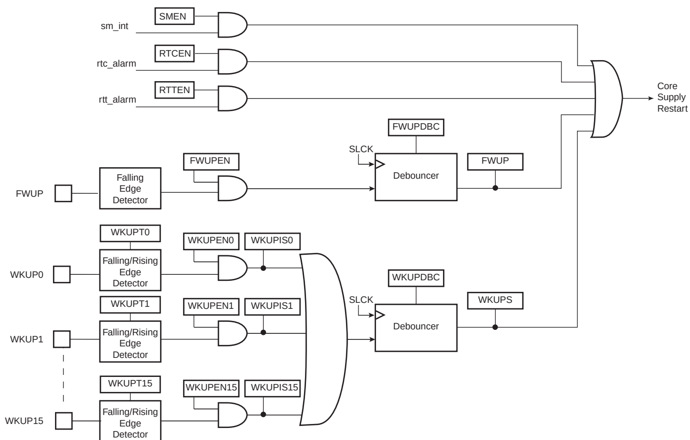
Figure 18-7. Wake Up Sources
