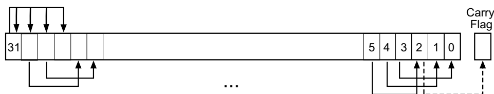
Figure 12-4. ASR #3
