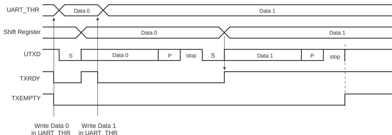
Figure 33-10. Transmitter Control
