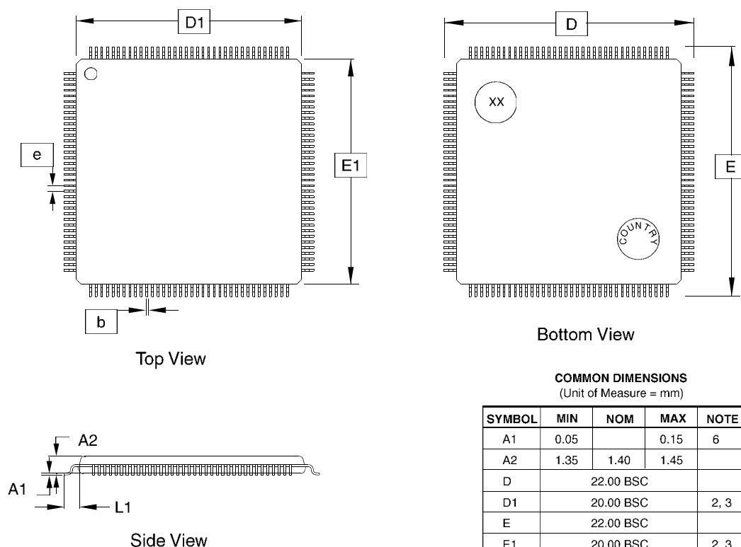
Figure 43-3. 144-lead LQFP Package Drawing
