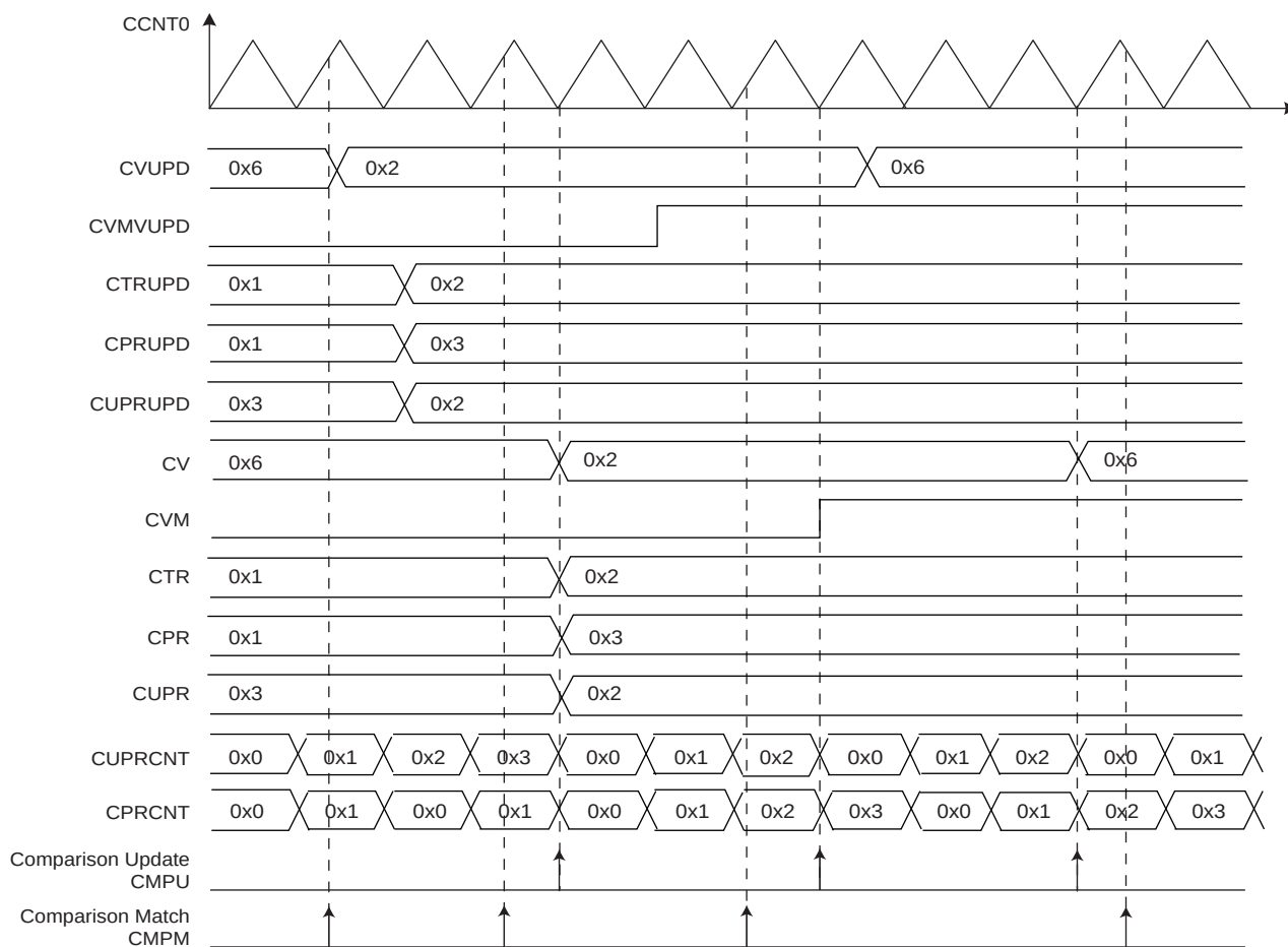
Figure 37-14. Comparison Waveform
