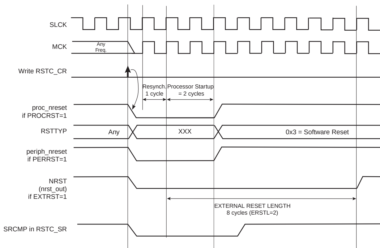
Figure 15-5. Software Reset
