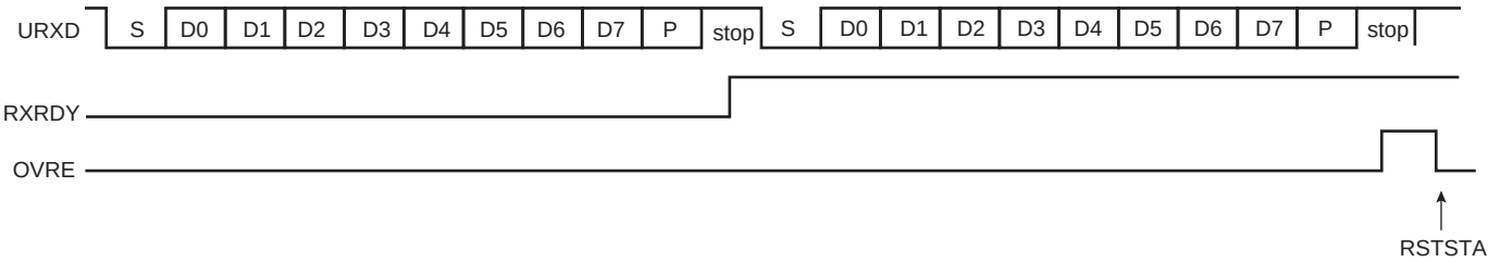
Figure 33-6. Receiver Overrun
