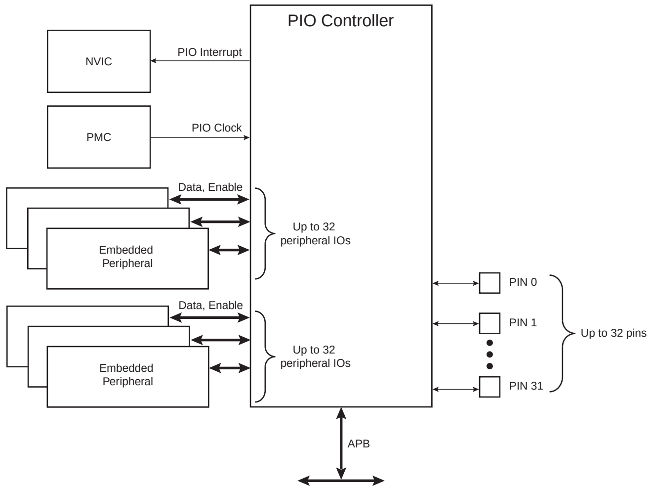
Figure 29-1. Block Diagram
