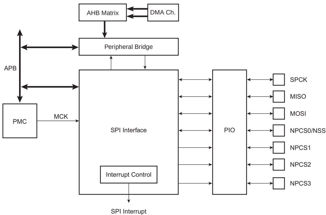
Figure 31-1. Block Diagram
