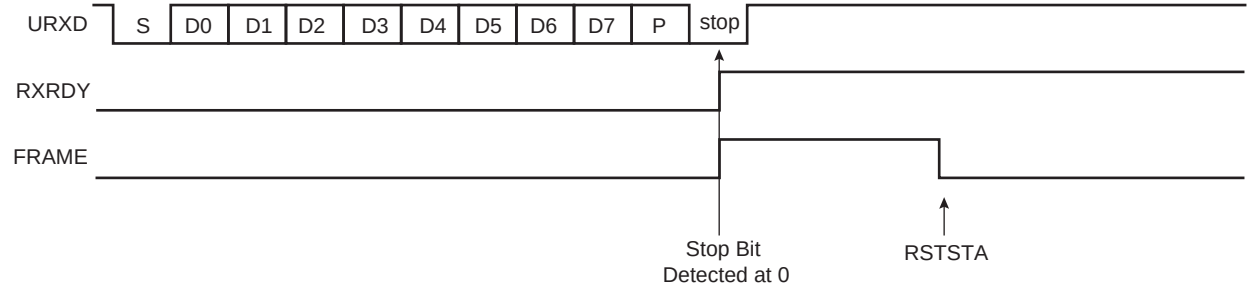
Figure 33-8. Receiver Framing Error
