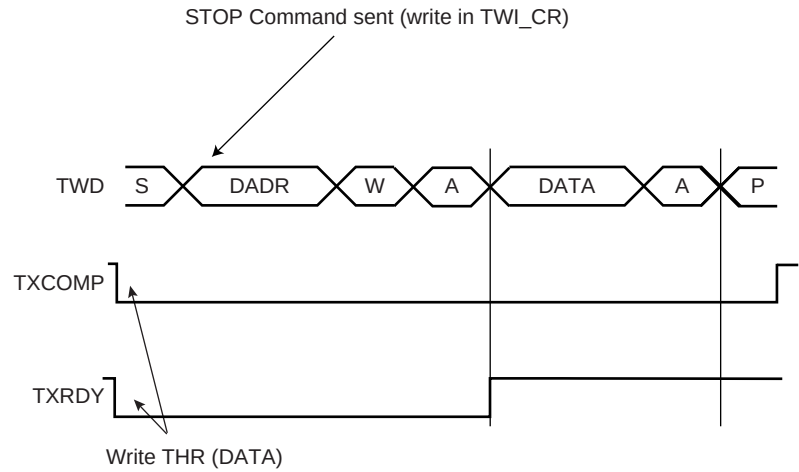
Figure 32-7. Master Write with Multiple Data Bytes
