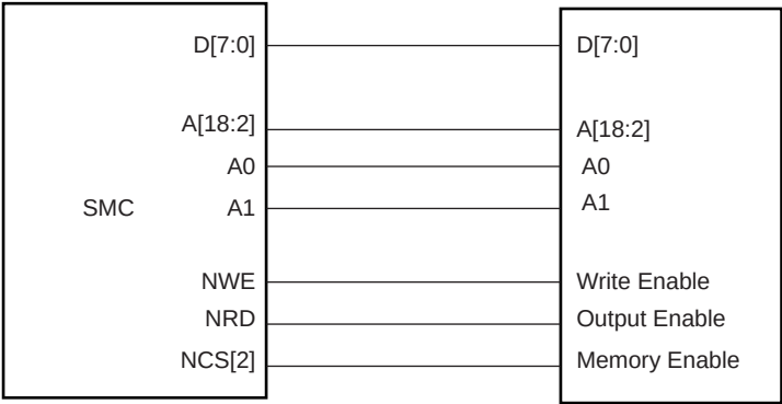
Figure 24-4. Memory Connection for an 8-bit Data Bus
