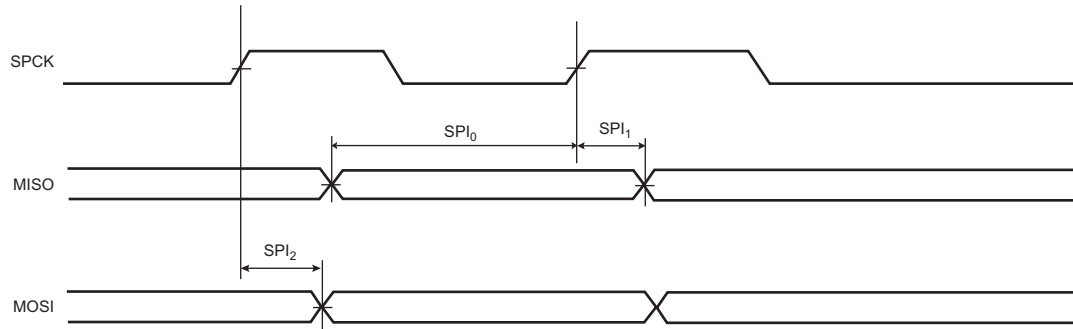
Figure 42-17. SPI Master Mode with (CPOL = NCPHA = 0) or (CPOL = NCPHA = 1)
