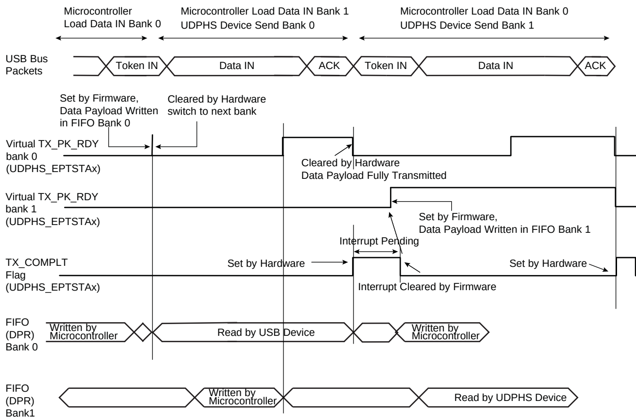
Figure 38-9. Data IN Transfer for Endpoint with Two Banks
