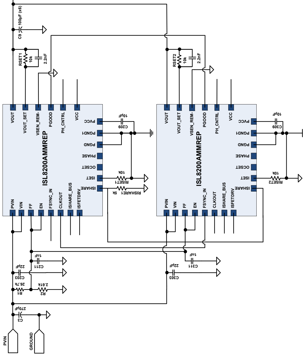
FIGURE 4. TWO PHASE 20A 3.3V OUTPUT CIRCUIT
