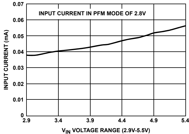
FIGURE 5. I_Q vs V_{IN} (PFM)
