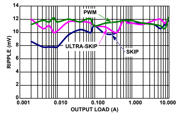
FIGURE 26. V_{OUT2} = 3.3V RIPPLE vs LOAD
