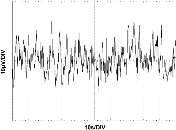
FIGURE 27. V_{OUT} NOISE
