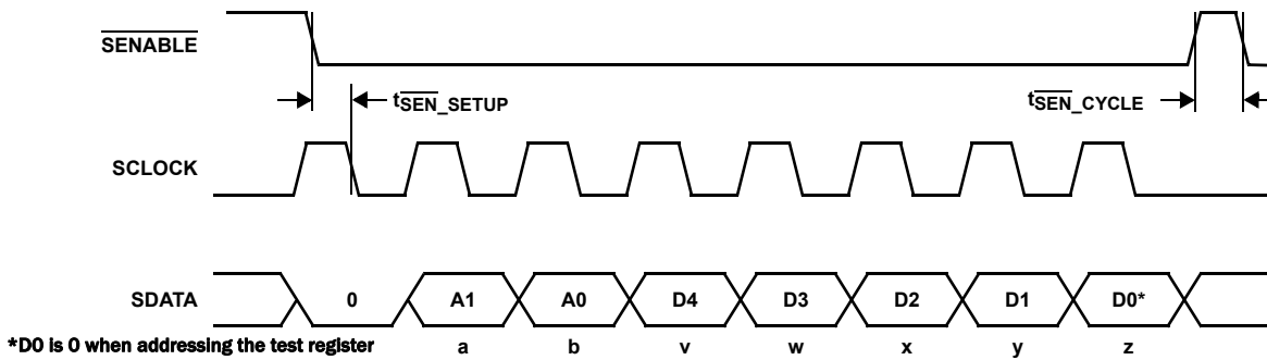
FIGURE 35. SERIAL TIMING
