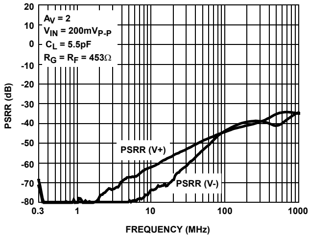
FIGURE 10. PSRR CHANNELS
