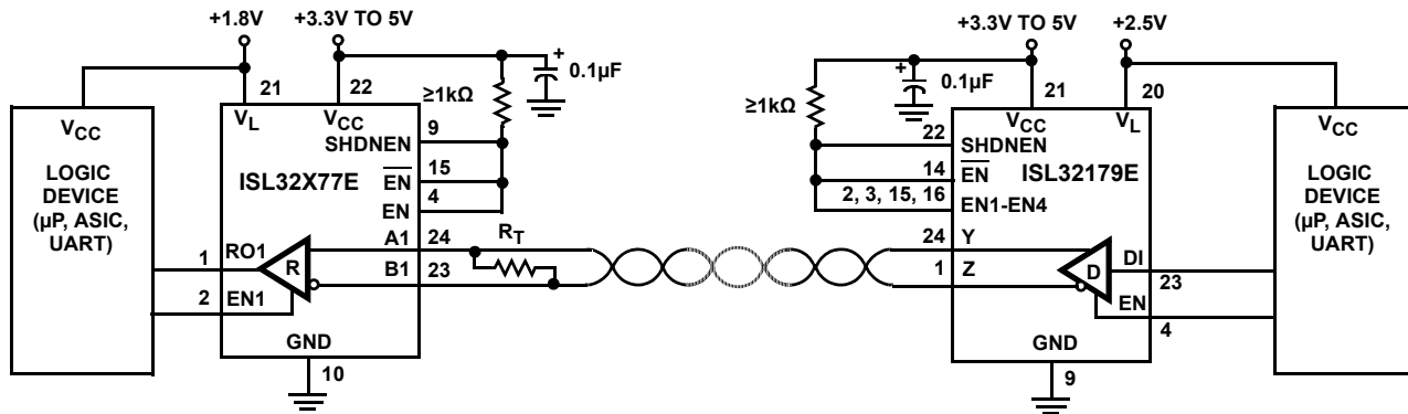
FIGURE 4. NETWORK USING PAIRED ENABLES
