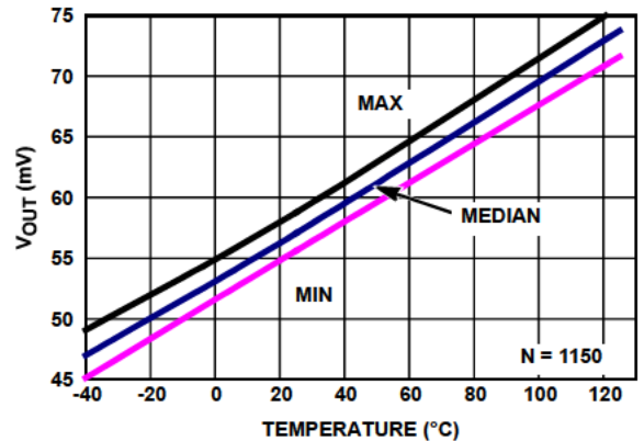
FIGURE 35. V_{OUT \text{ LOW}} vs TEMPERATURE V_+, V_- = \pm 2.5V, R_L = 1k
