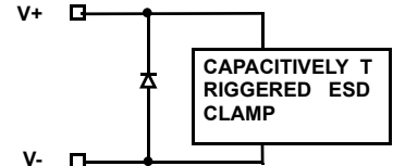
CIRCUIT 3
