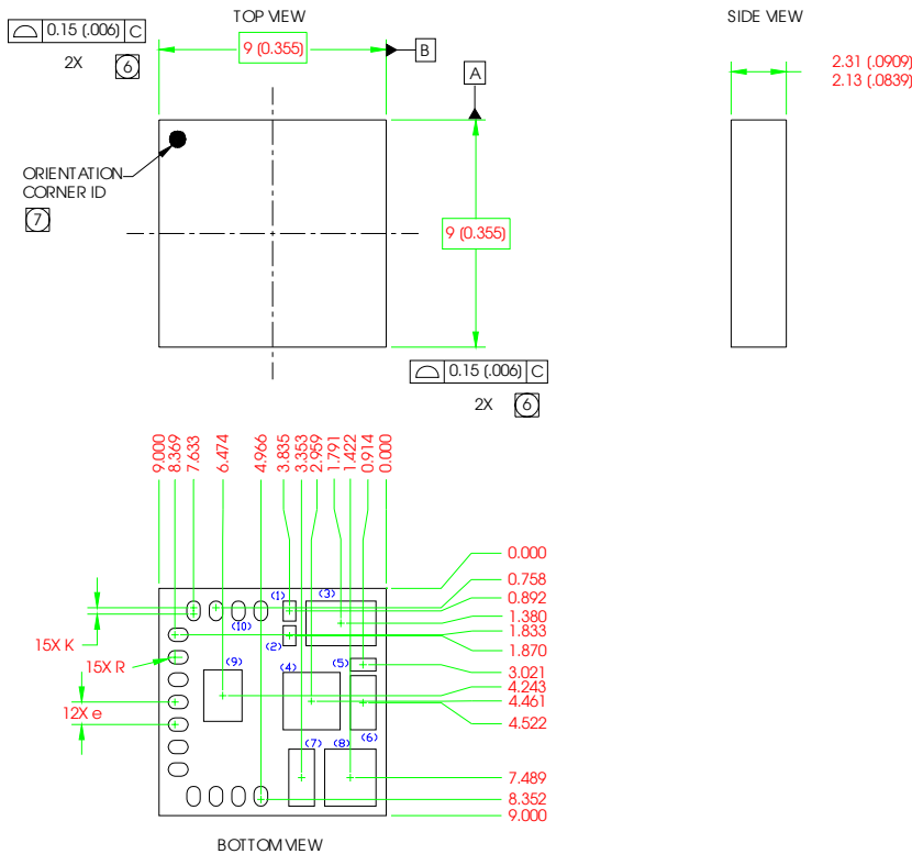
Fig. 25: Outline Drawing
