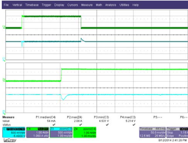
Figure 22 – Transient Response (4.5 V_{\text{MIN}} ). 85 VAC, 0-2 A Load Step. Upper: I_{\text{LOAD}} , 1 A / div. Lower: V_{\text{OUT}} , 500 mV, 50 ms / div.
