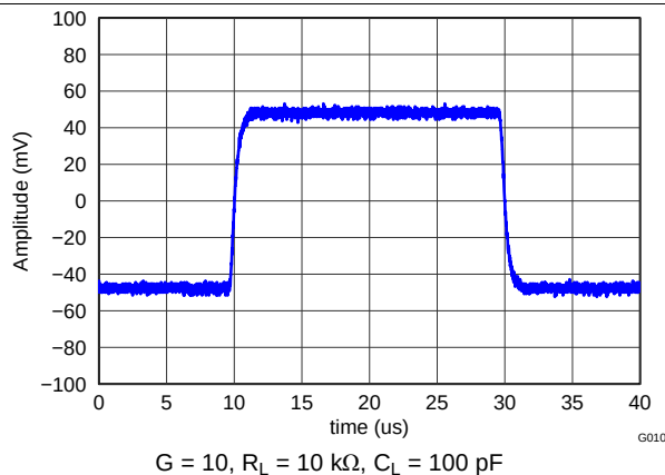
Figure 53. Small-Signal Response
