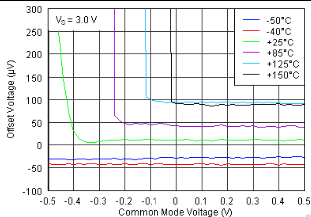
Figure 43. Offset Voltage vs Negative Common-Mode Voltage
