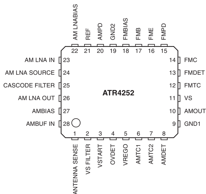
Figure 2-1. Pinning VQFN 4x5 / 28L
