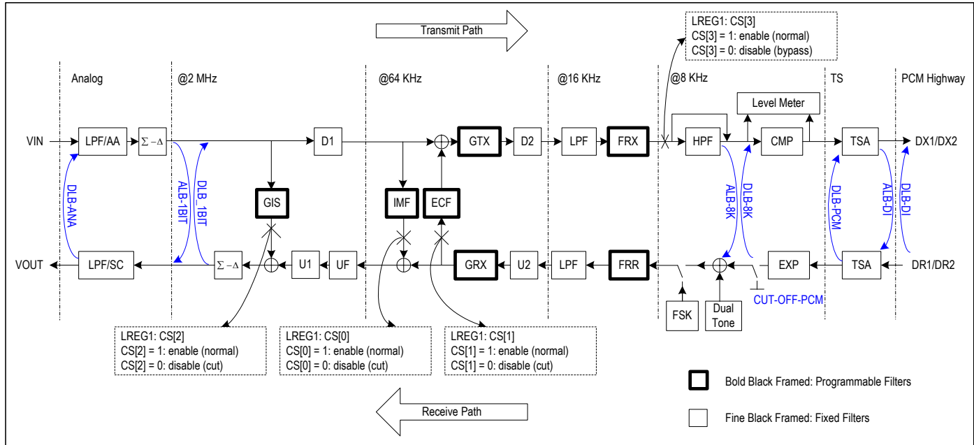
Figure - 4 Signal Flow for Each Channel
