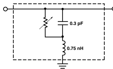
Figure 21. Equivalent Circuit.
