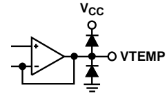
Figure 6. VTEMP Interface
