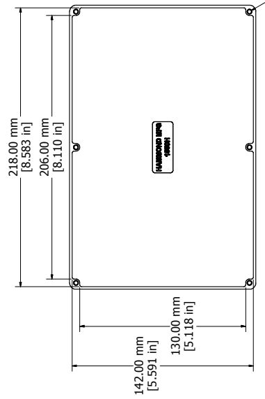
Top View Looking Inside Box
