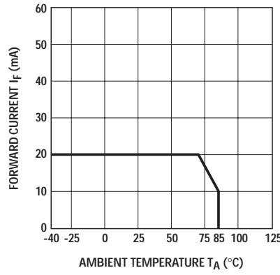
Figure 12. LED forward current vs. ambient temperature, HCPL-3101.
