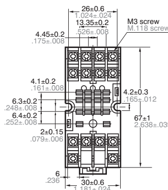
External dimensions
