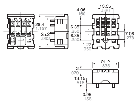
External dimensions
