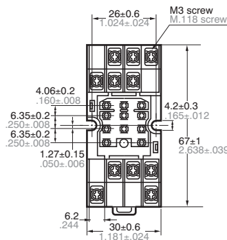
External dimensions
