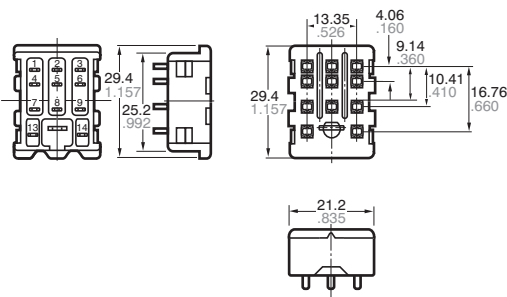
External dimensions
